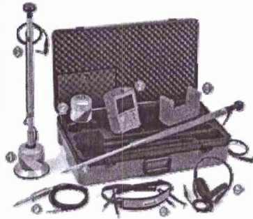
NETWORK TECHNICIANS' LEAK KIT
